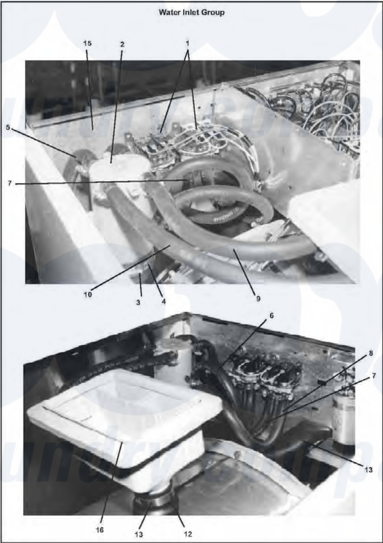
Dexter Commercial Dexter WCN18AA Washer Parts Parts Diagram Water Inlet Group Click on the part number to view part
