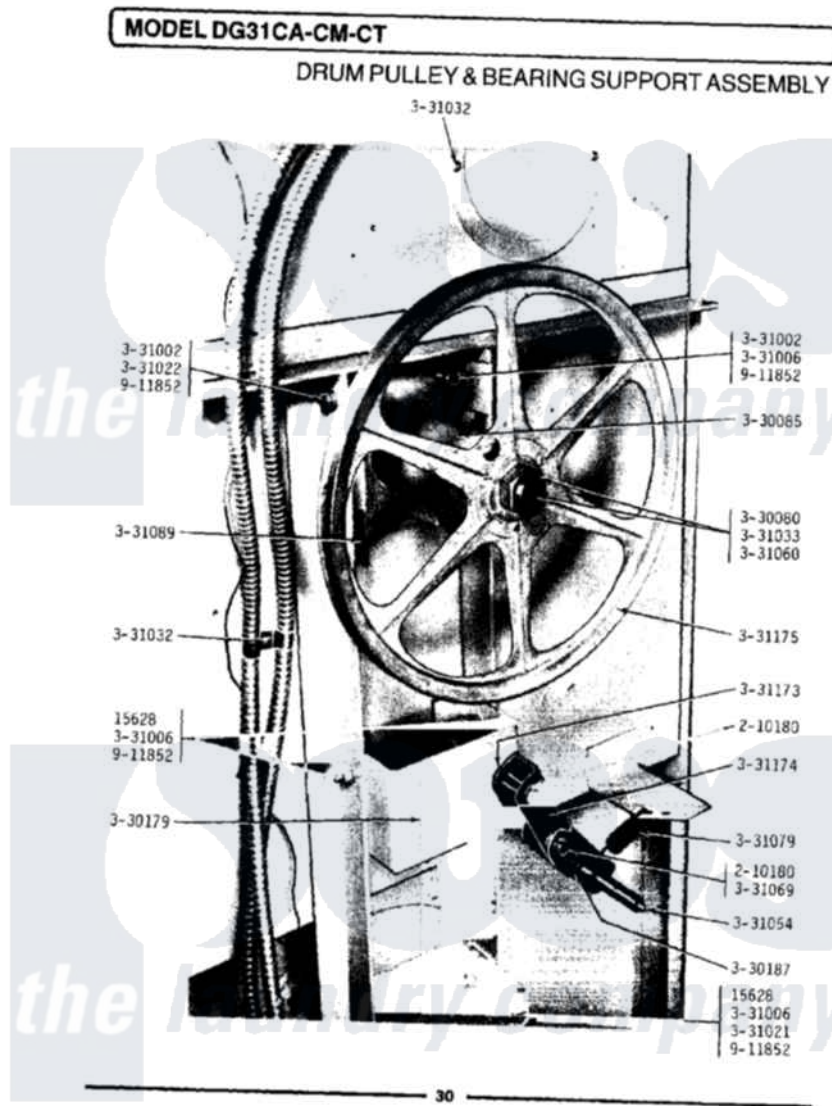
Maytag Commercial Maytag DG31CM Dryer Parts Parts Diagram 12 - DRUM PULLEY & BEARING SUPPORT ASSEMBLY
