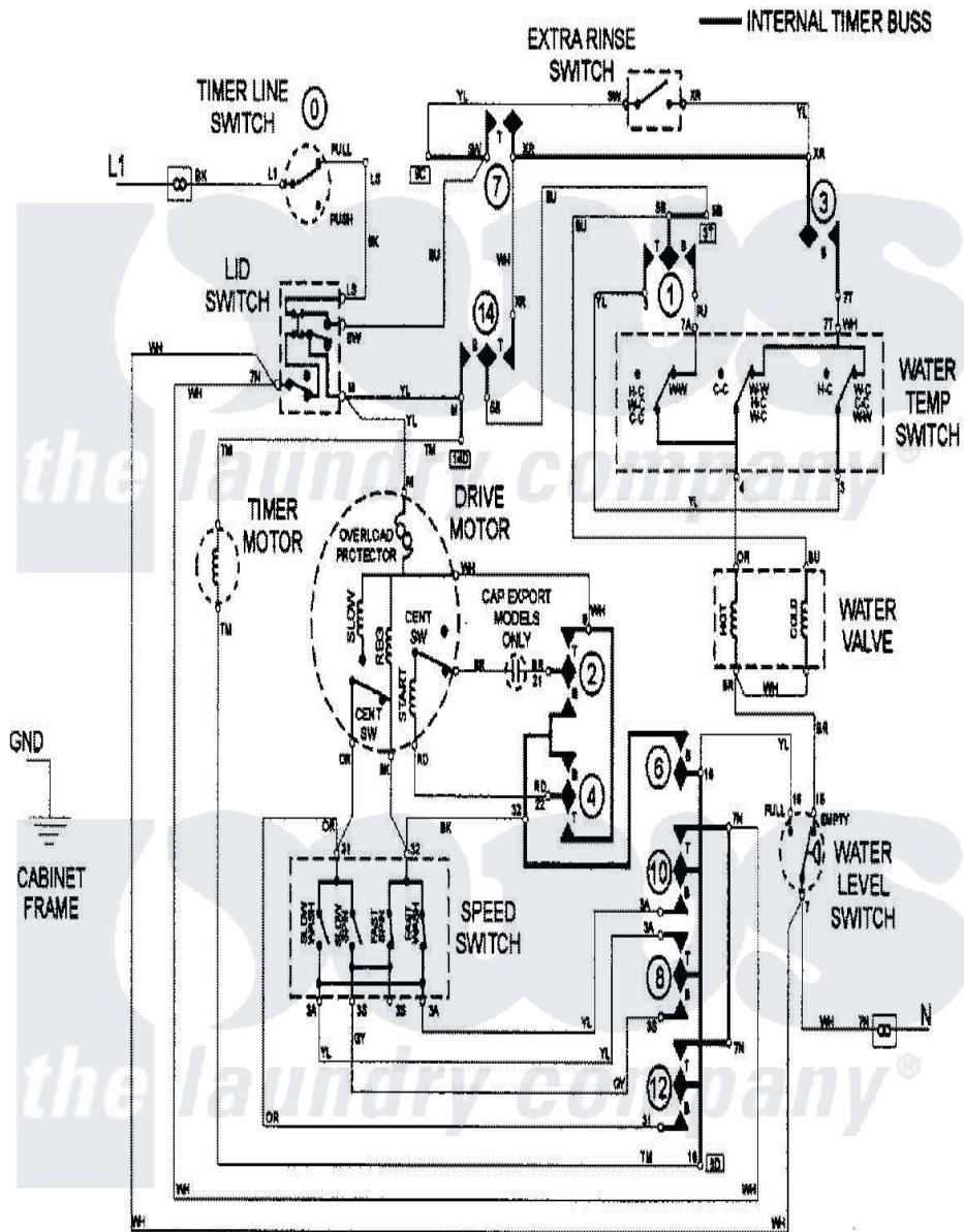
Maytag Residential Maytag LAT3500AAQ Washer Parts Parts Diagram 08 - WIRING INFORMATION Click on the part number to view part
