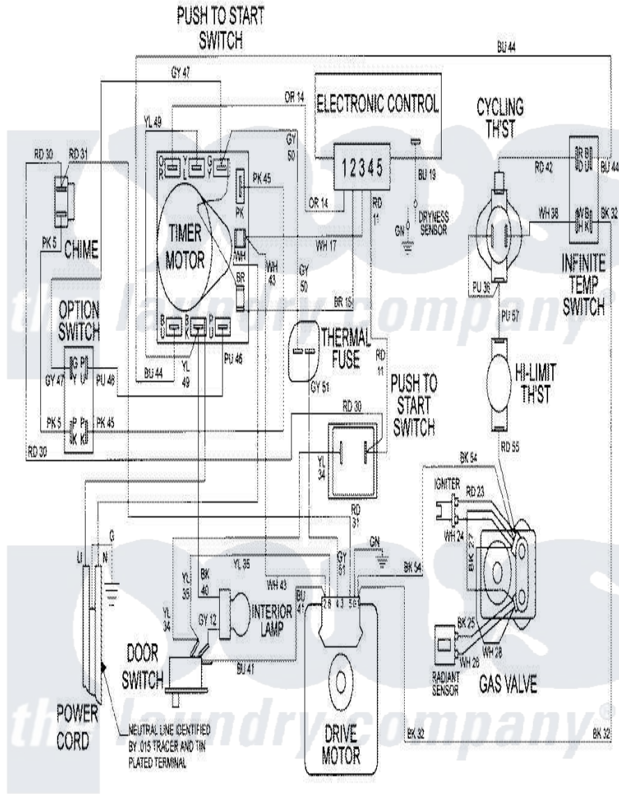
Maytag Residential Maytag MDG3000AXQ Dryer Parts Parts Diagram 08 - WIRING INFORMATION (MDG3000AXQ/AWQ)
