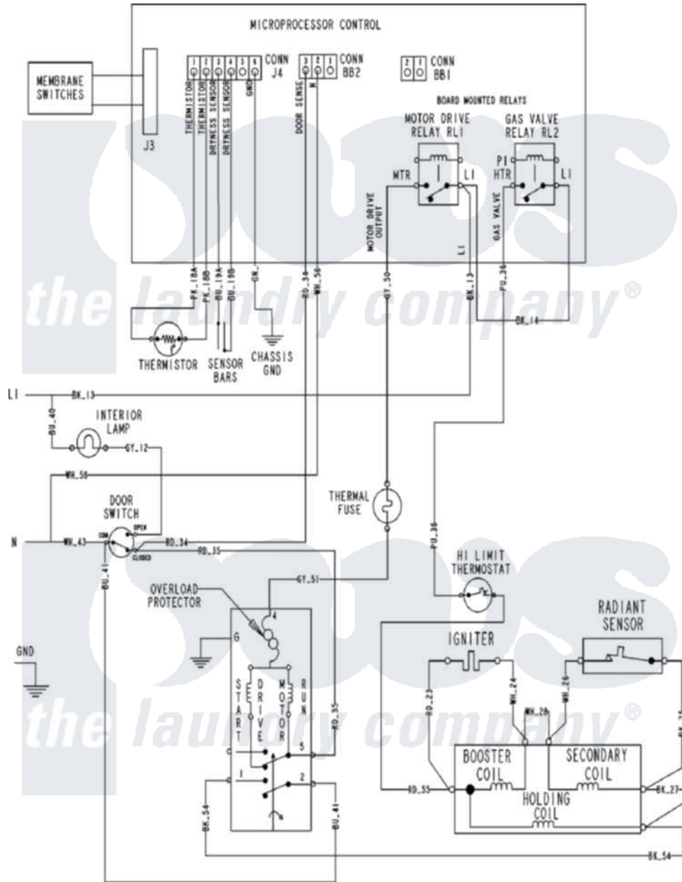
Maytag Residential Maytag MDG5500AWW Dryer Parts Parts Diagram 11 - WIRING INFORMATION SERIES 62 AND ABOVE
