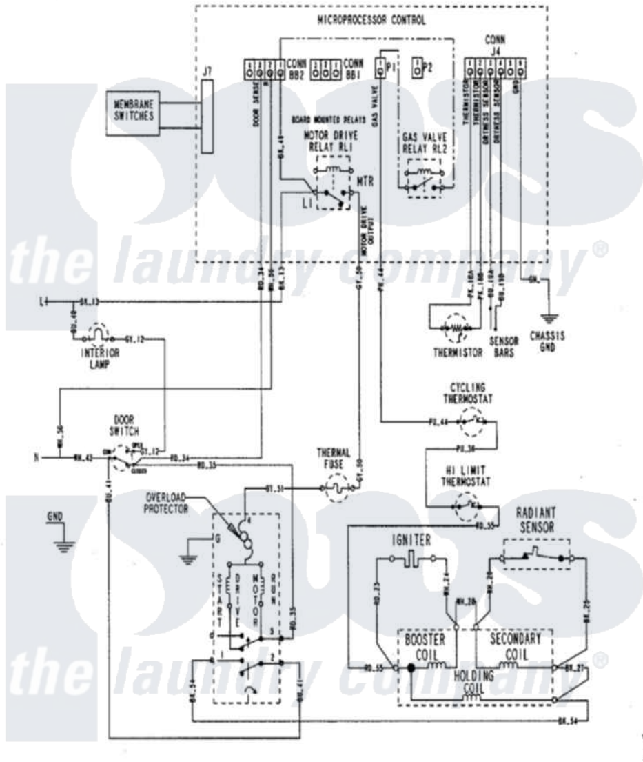
Maytag Residential Maytag MDG7500AWW Dryer Parts Diagram 10 - WIRING INFORMATION (AT SERIES 34)
