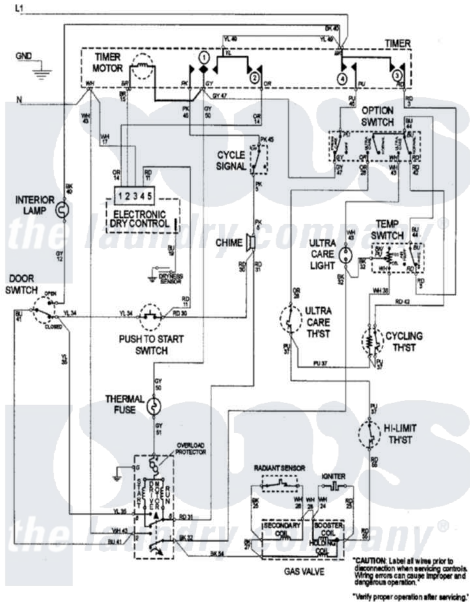
Maytag Residential Maytag MDG8000AWQ Dryer Parts Parts Diagram 06 - WIRING INFORMATION Click on the part number to view part
