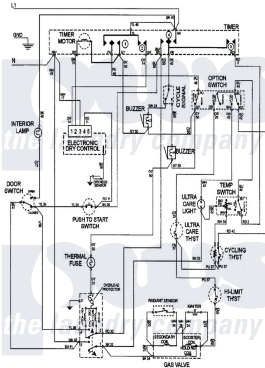
Maytag Residential Maytag MDG8057BWW Dryer Parts Parts Diagram 08 - WIRING INFORMATION Click on the part number to view part
