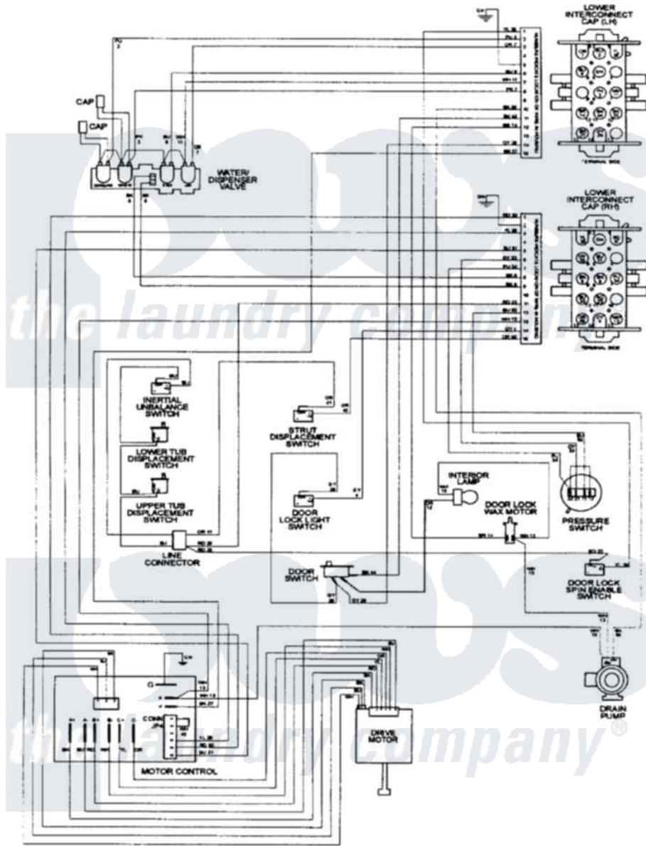
Maytag Residential Maytag MHW2000AWW Stacked Washer and Dryer Parts Parts Diagram 18 - WIRING INFORMATION
