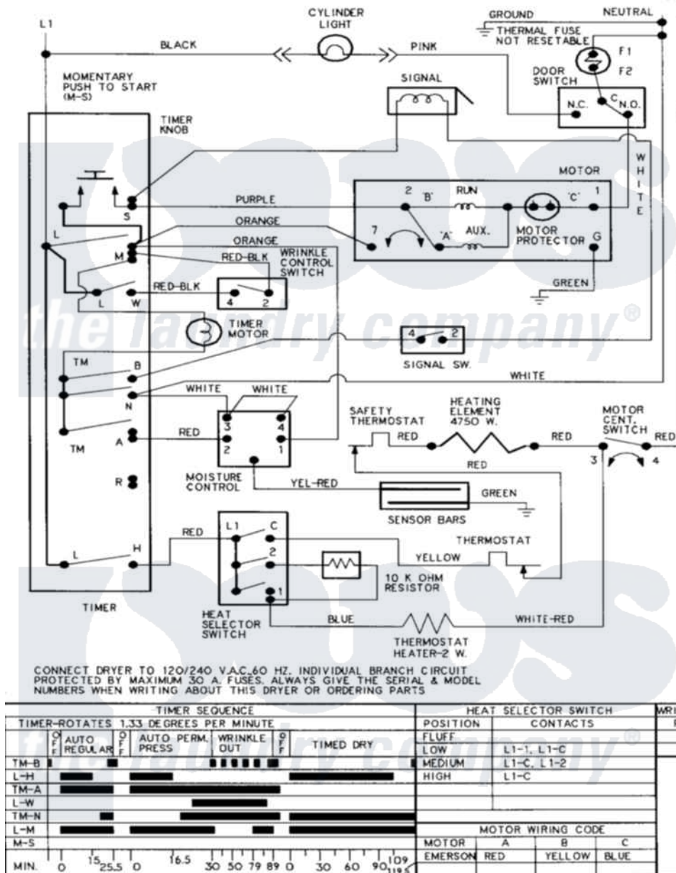
Maytag Residential Maytag PYET444AYW Dryer Parts Parts Diagram 10 - WIRING INFORMATION (SERIES 13) Click on the part number to view part
