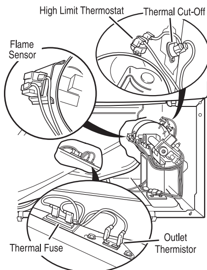
Gas Dryer
