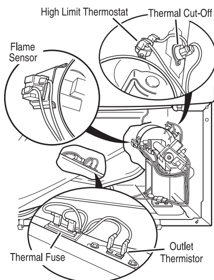
Gas Dryer
