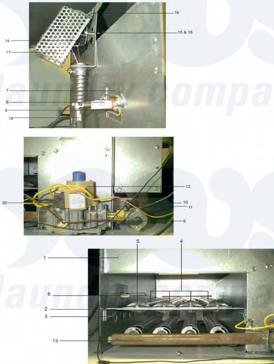
Dexter Commercial Dexter DTCK80 Dryer Parts Parts Diagram Burner Housing Group Click on the part number to view part
