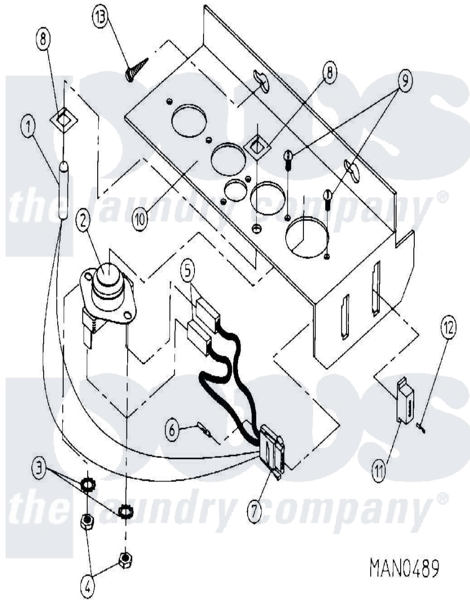
Maytag Commercial Maytag DG75PN1 Dryer Parts Parts Diagram 14 - MICROPORCESSOR SENSOR BRACKET (DG75PN1)
