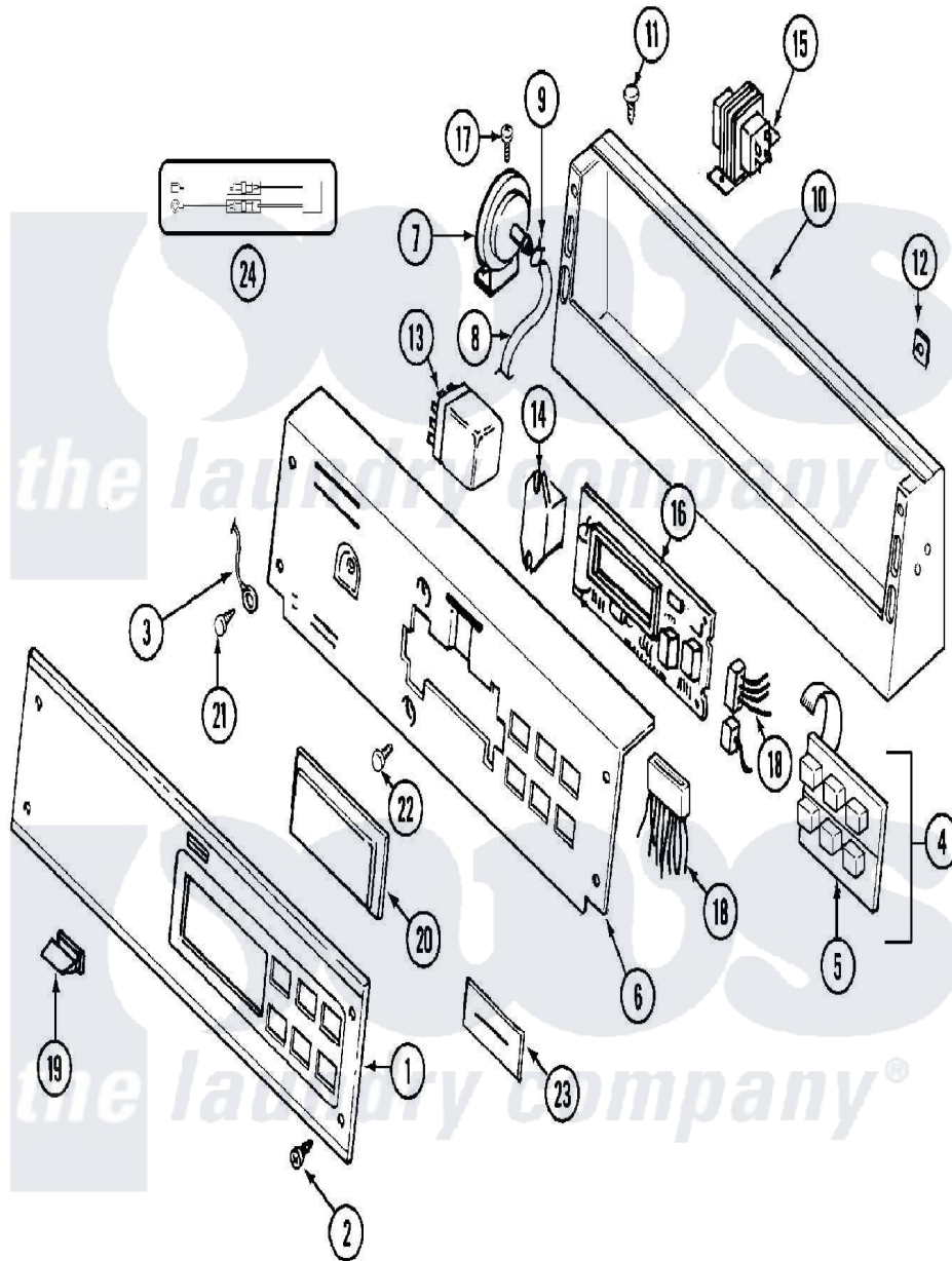
Maytag Commercial Maytag MAT12PRSAW Washer Parts Parts Diagram 01 - CONTROL PANEL Click on the part number to view part
