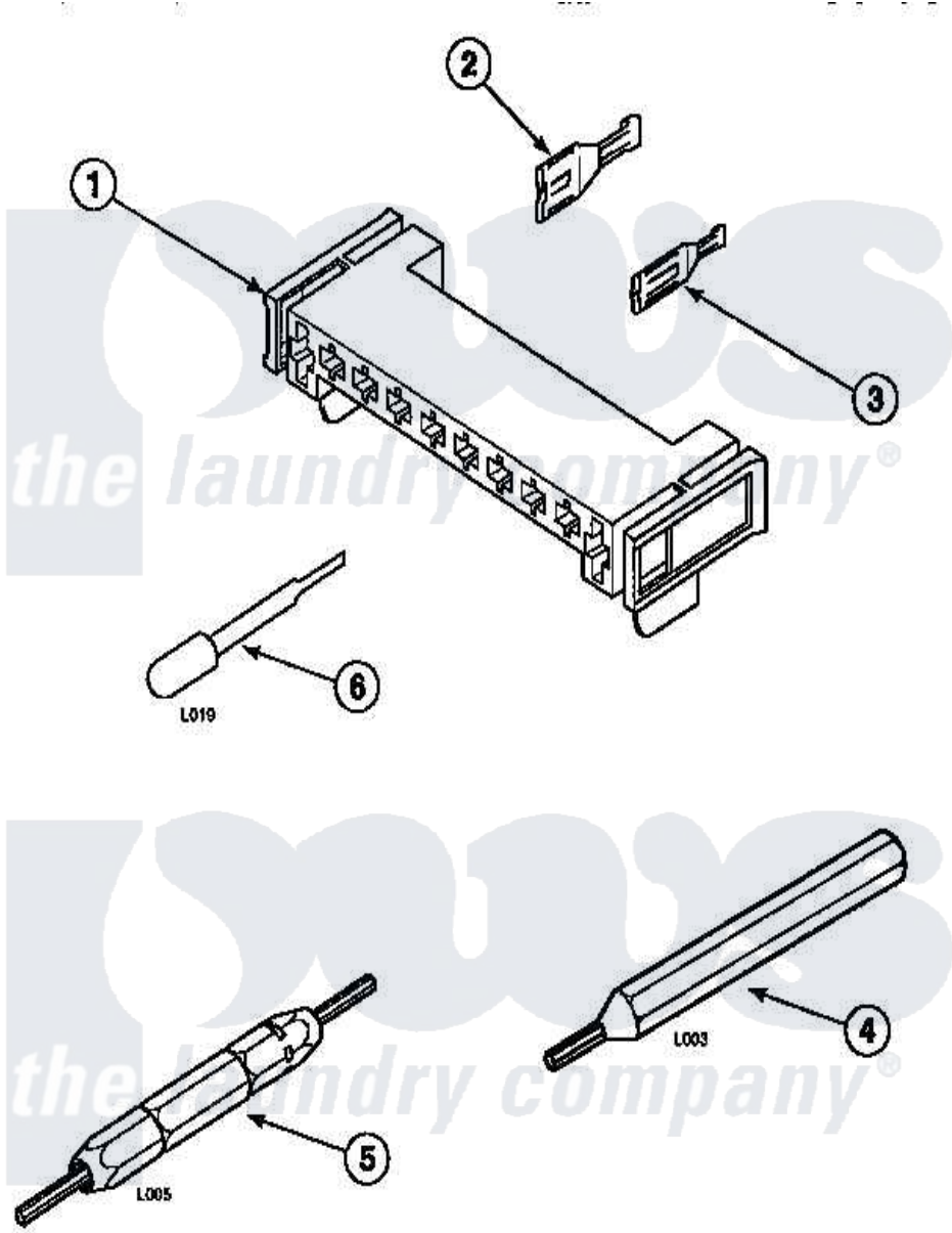
Amana Residential Amana LG9209W2 (BOM: PLG9209W2) Dryer Parts Diagram 16 - Page 21 Click on the part number to view part
