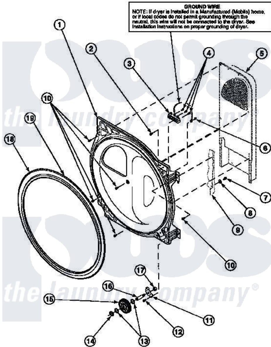
Amana Residential Amana LG9209W2 (BOM: PLG9209W2) Dryer Parts Parts Diagram 19 - REAR BLKHD/SEAL/CYLINDER ROLLER/TERM BLK Click on the part number to view part
