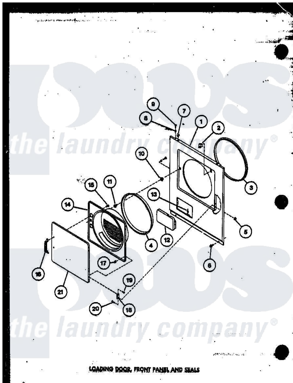
Amana Residential Amana TGA600 (BOM: P7575202W) Dryer Parts Parts Diagram 08 - LOADING DOOR Click on the part number to view part
