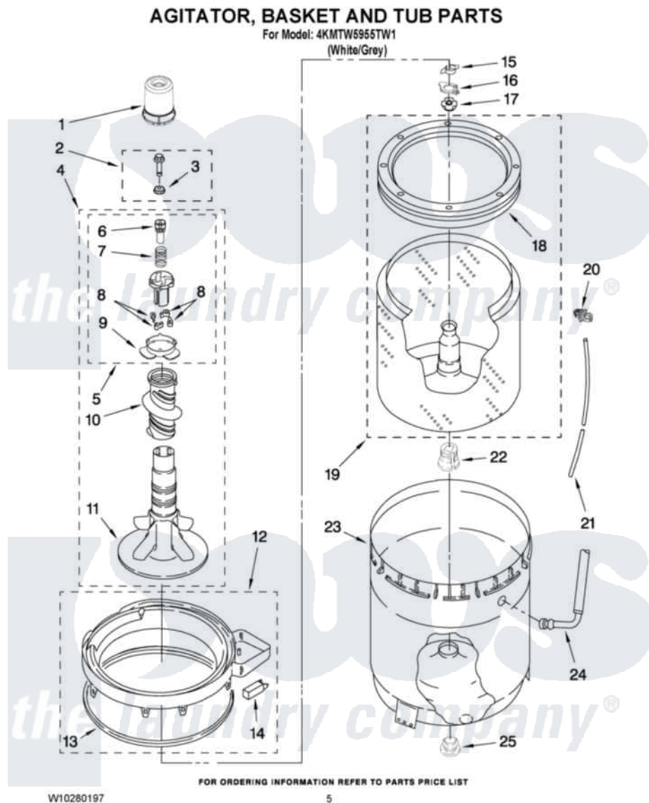
Maytag Residential Maytag 4KMTW5955TW1 Washer Parts Parts Diagram 03 - AGITATOR, BASKET AND TUB PARTS
