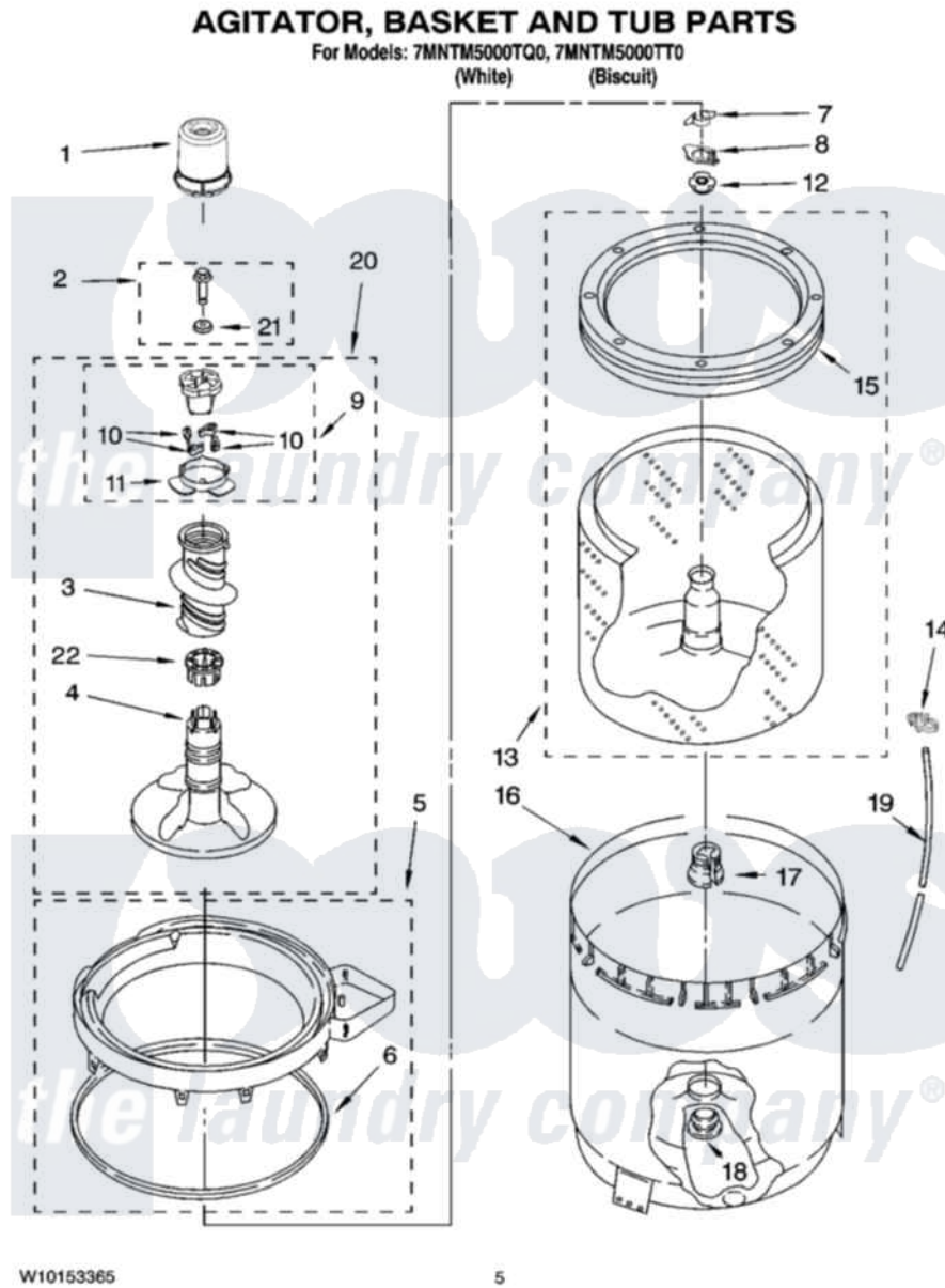
Maytag Residential Maytag 7MNTM5000TQ0 Washer Parts Parts Diagram 03 - AGITATOR, BASKET AND TUB PARTS
