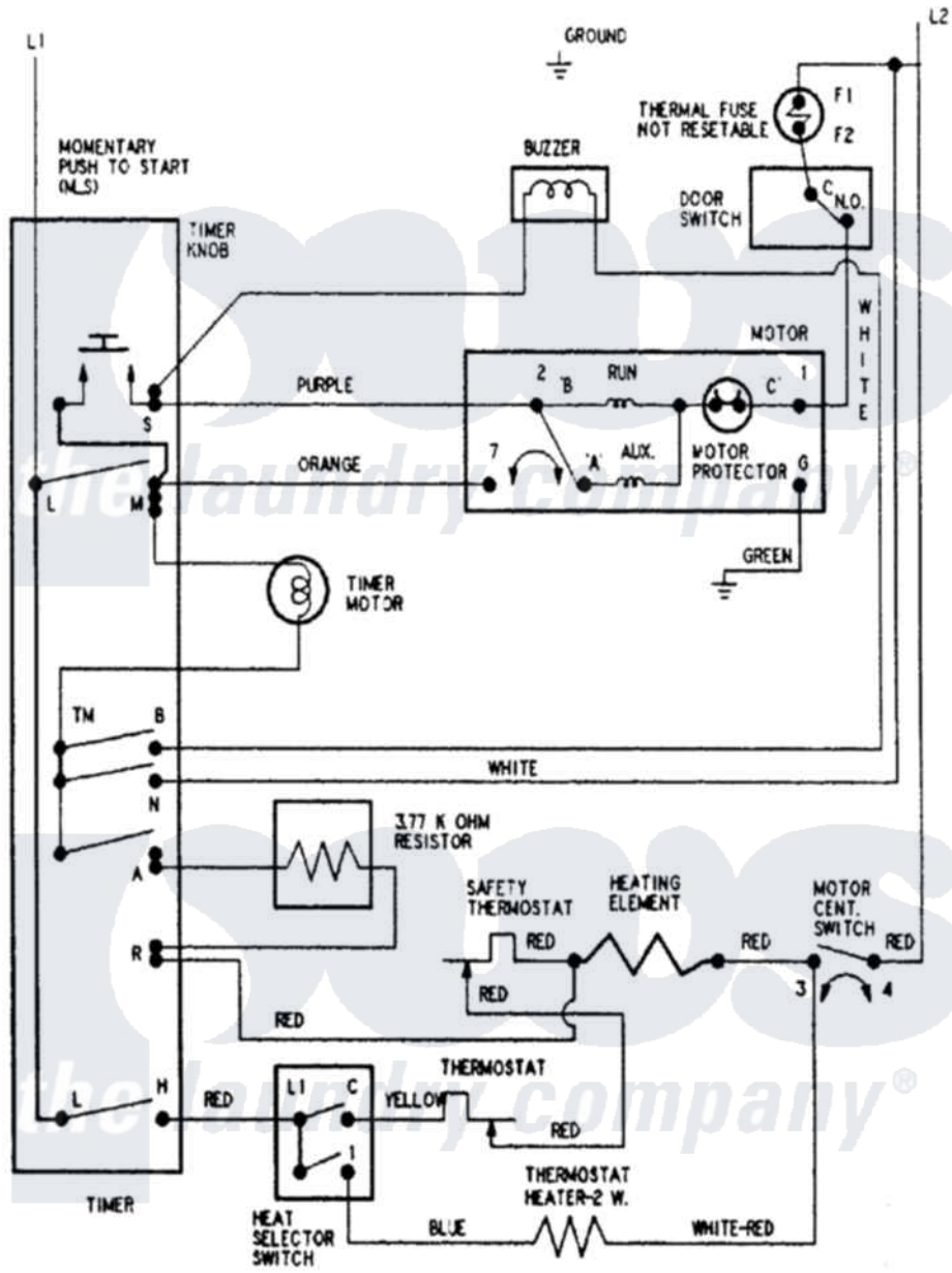
Maytag Residential Maytag CYE3004AGW Dryer Parts Parts Diagram 08 - WIRING INFORMATION Click on the part number to view part
