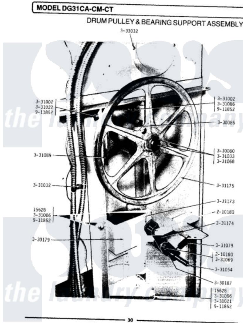
Maytag Residential Maytag DG31CM Dryer Parts Parts Diagram 12 - DRUM PULLEY & BEARING SUPPORT ASSEMBLY
