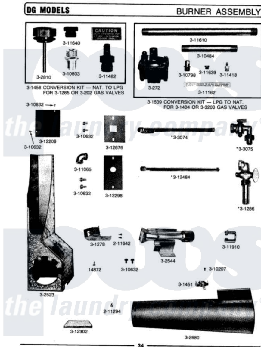
Maytag Residential Maytag DG606 Dryer Parts Parts Diagram 02 - BURNER ASSEMBLY Click on the part number to view part
