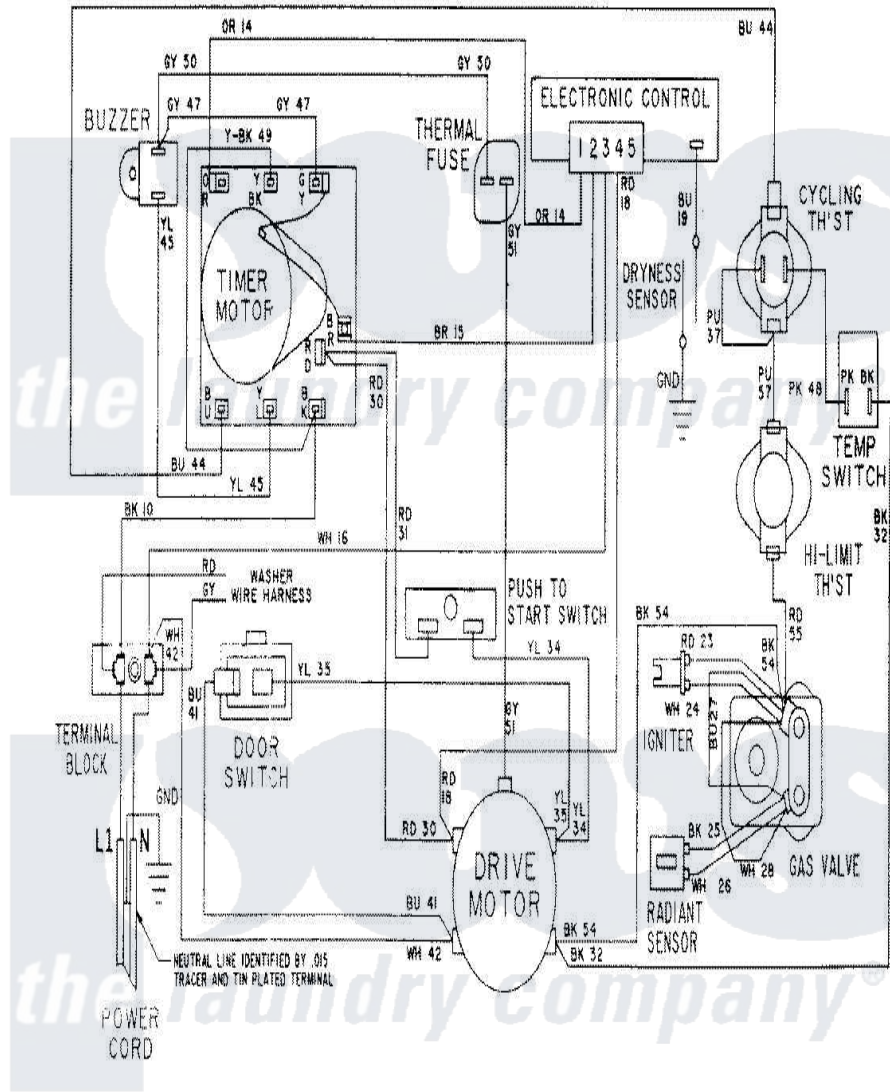
Maytag Residential Maytag LSG7804AAL Stacked Washer and Dryer Parts Parts Diagram 15 - WIRING INFORMATION-DRYER Click on the part number to view part
