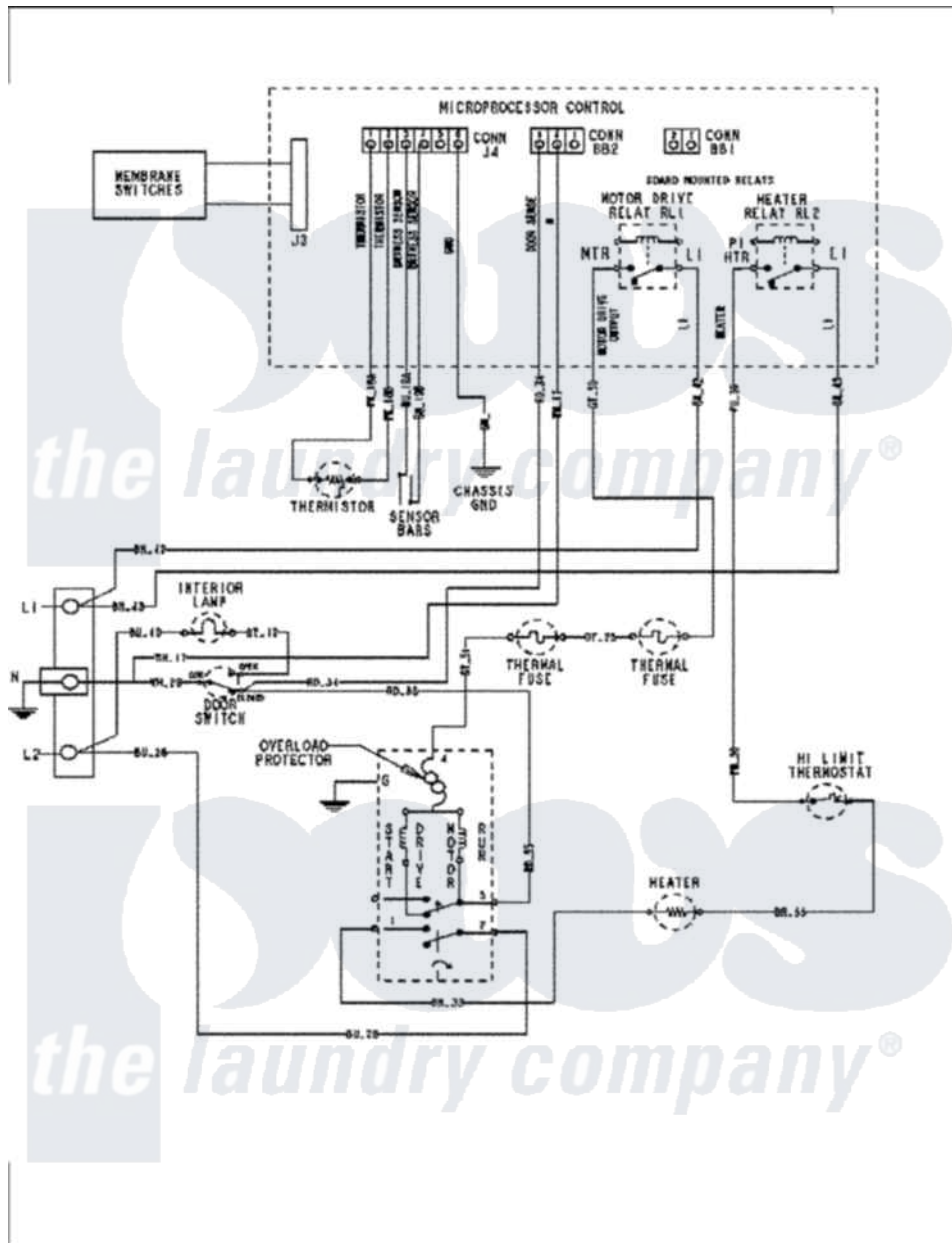
Maytag Residential Maytag MDE5500AZQ Dryer Parts Parts Diagram 09 - WIRING INFORMATION SERIES 62 AND LATER
