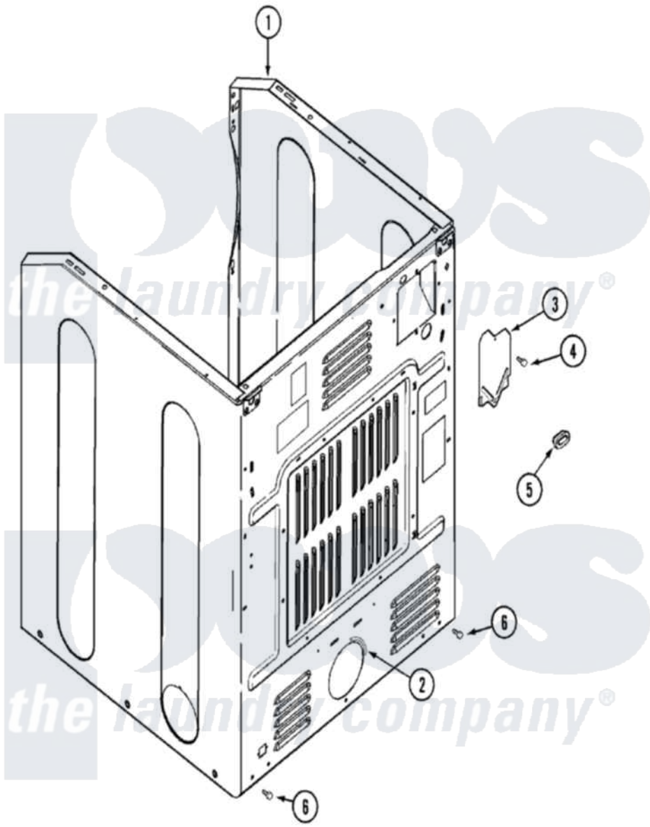
Maytag Residential Maytag MDE7500AYQ Dryer Parts Parts Diagram 01 - CABINET-REAR Click on the part number to view part
