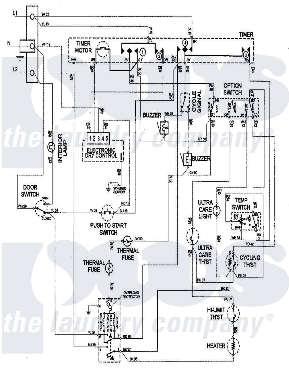
Maytag Residential Maytag MDE8057AYW Dryer Parts Parts Diagram 08 - WIRING INFORMATION Click on the part number to view part
