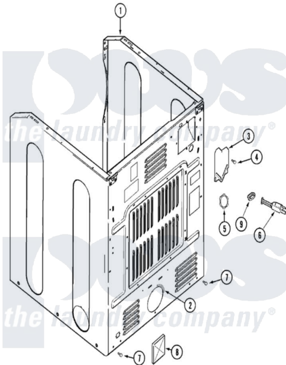
Maytag Residential Maytag MDE8757AYQ Dryer Parts Parts Diagram 02 - CABINET-REAR Click on the part number to view part
