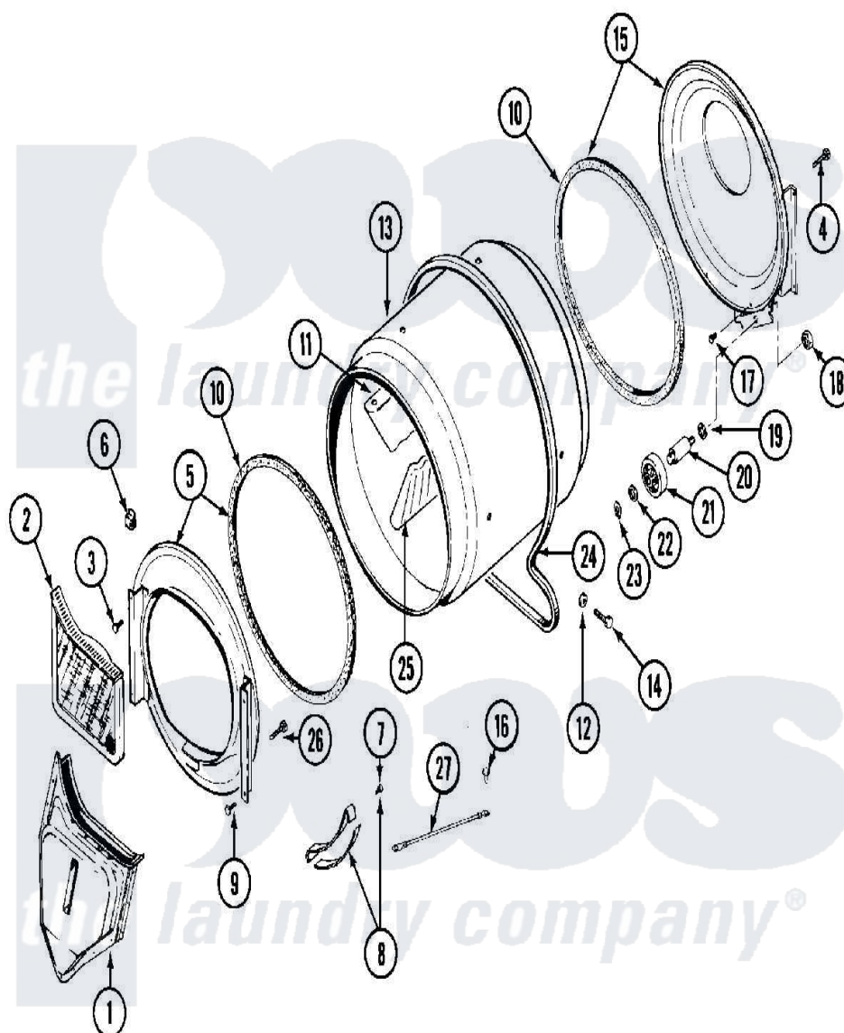
Maytag Residential Maytag MDG13PDAGW Dryer Parts Parts Diagram 05 - TUMBLER Click on the part number to view part
