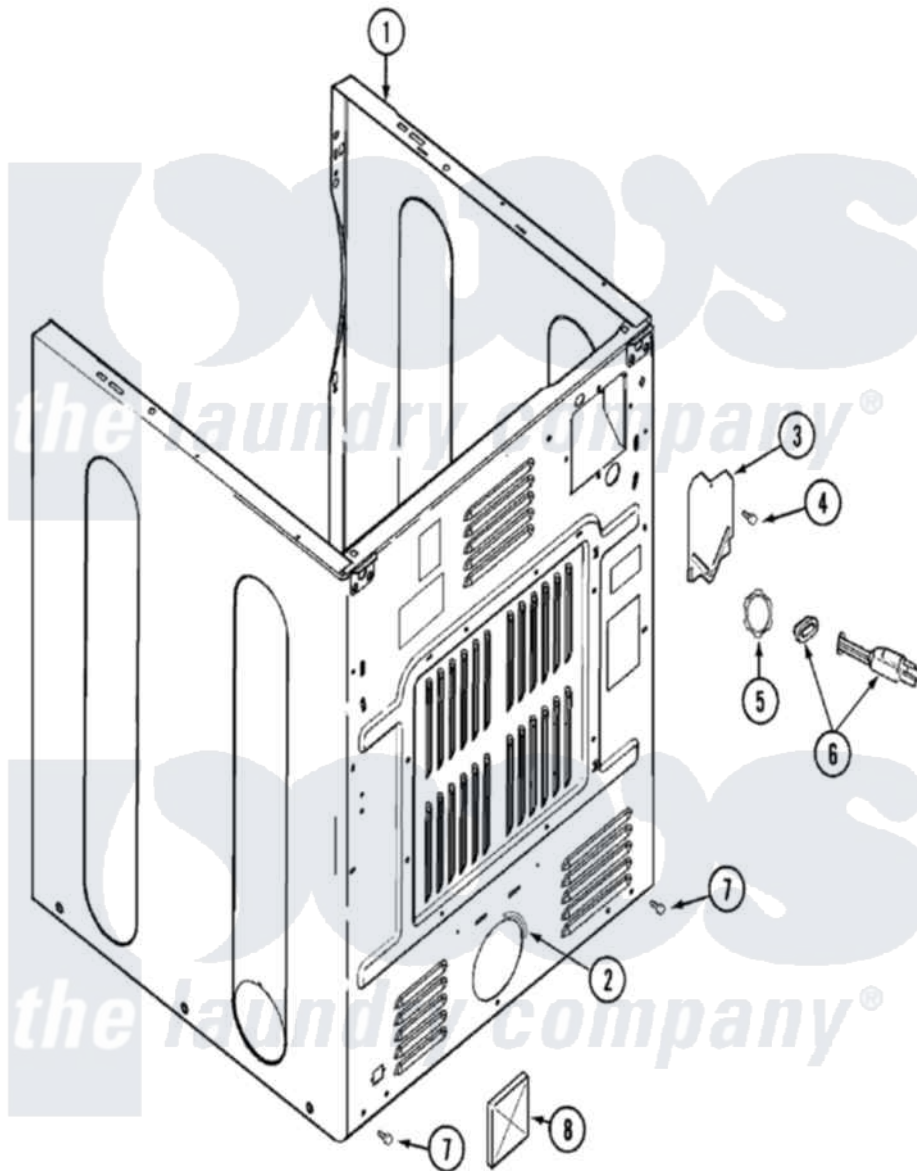
Maytag Residential Maytag MDG5960BWW Dryer Parts Parts Diagram 02 - CABINET-REAR Click on the part number to view part
