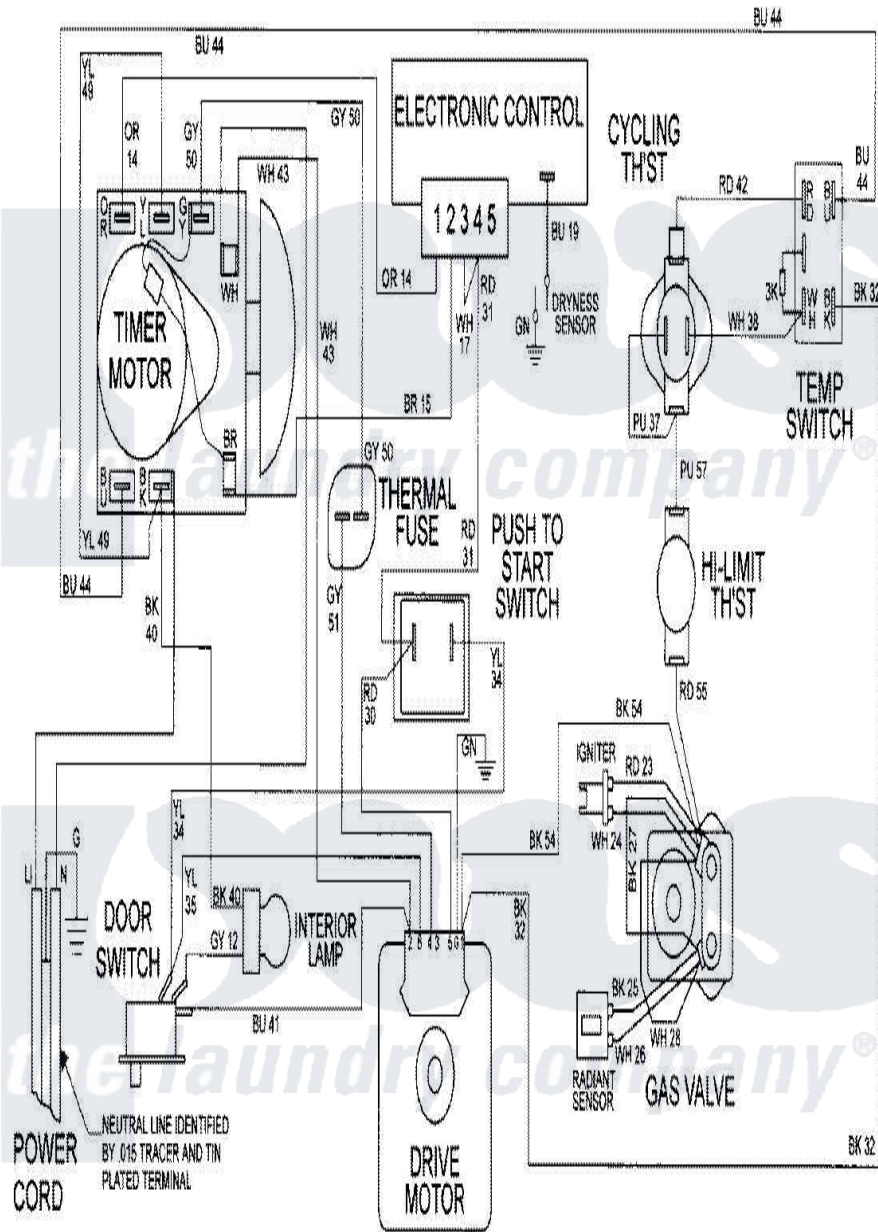
Maytag Residential Maytag MDG5960BWW Dryer Parts Parts Diagram 08 - WIRING INFORMATION Click on the part number to view part
