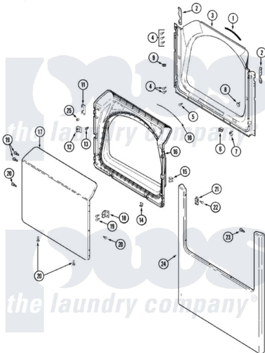
Maytag Residential Maytag MDG7057AWQ Dryer Parts Parts Diagram 02 - DOOR Click on the part number to view part
