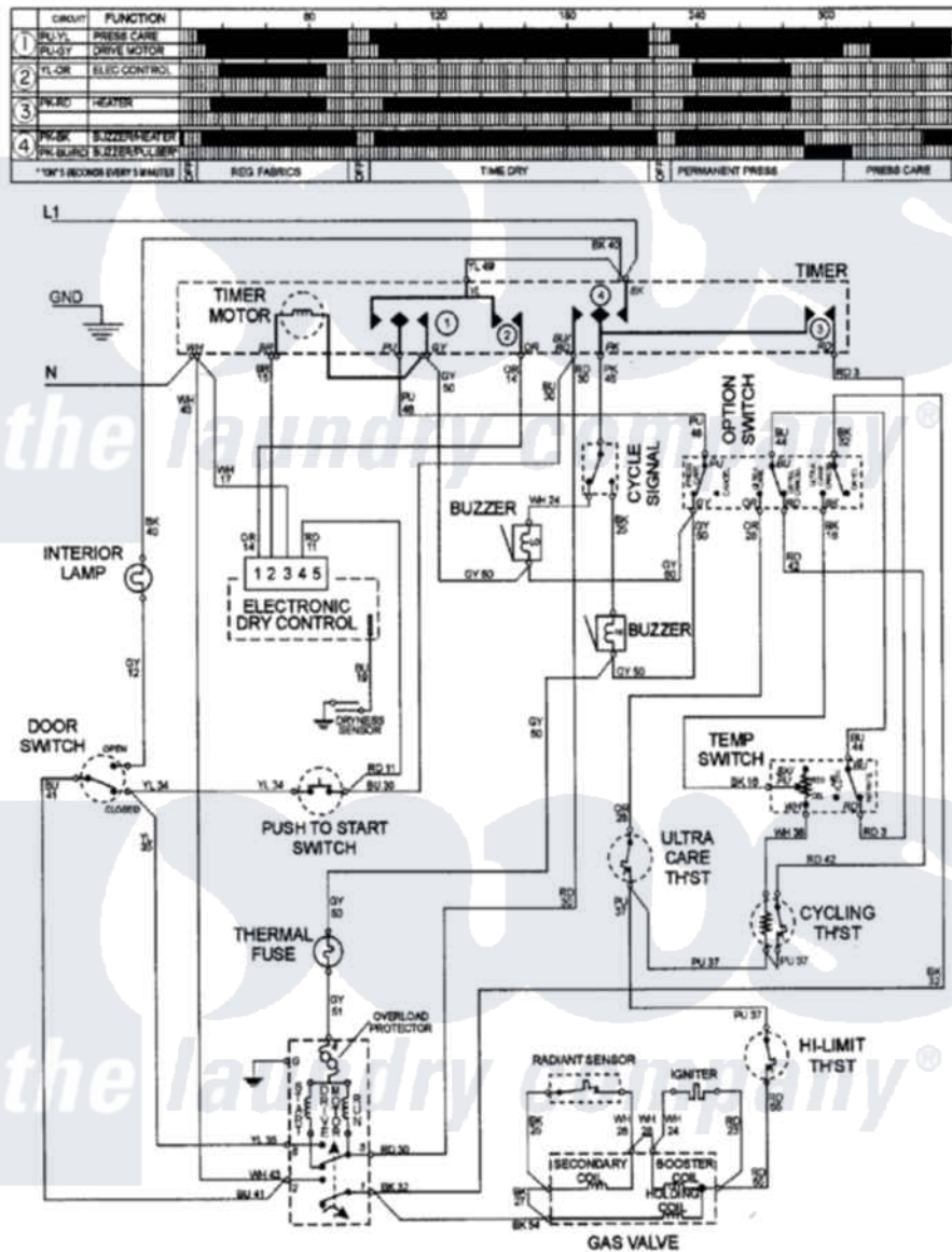
Maytag Residential Maytag MDG8058BWW Dryer Parts Parts Diagram 08 - WIRING INFORMATION Click on the part number to view part
