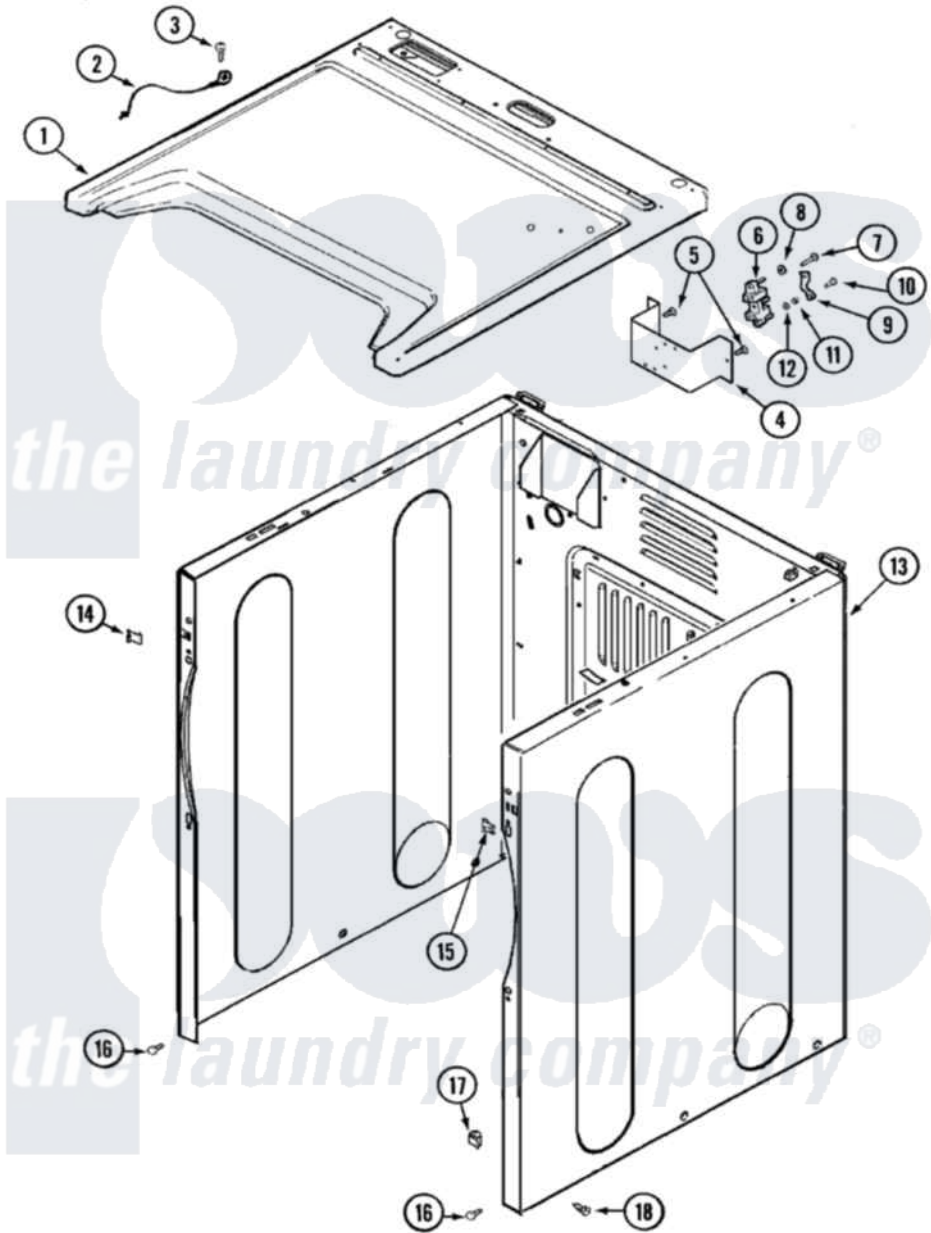
Maytag Residential Maytag MDG8506AWW Dryer Parts Parts Diagram 01 - CABINET Click on the part number to view part
