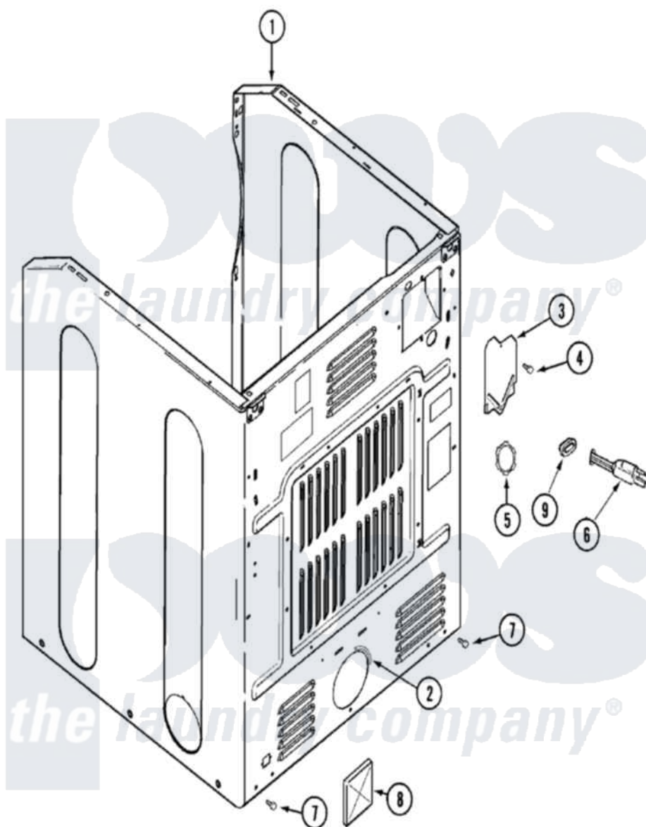
Maytag Residential Maytag MDG8757AWQ Dryer Parts Parts Diagram 02 - CABINET-REAR Click on the part number to view part
