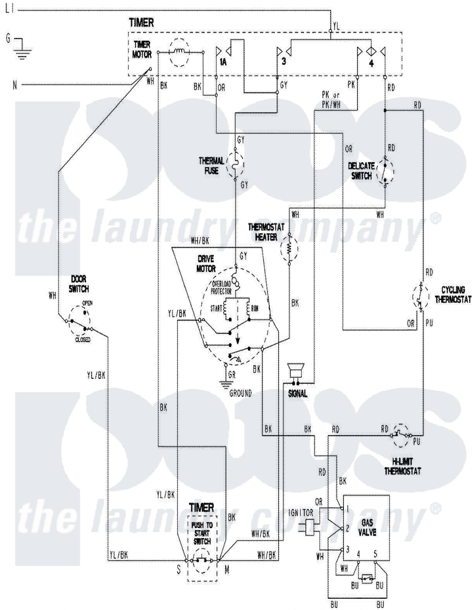
Maytag Residential Maytag PDGT910AWW Dryer Parts Parts Diagram 06 - WIRING INFORMATION Click on the part number to view part
