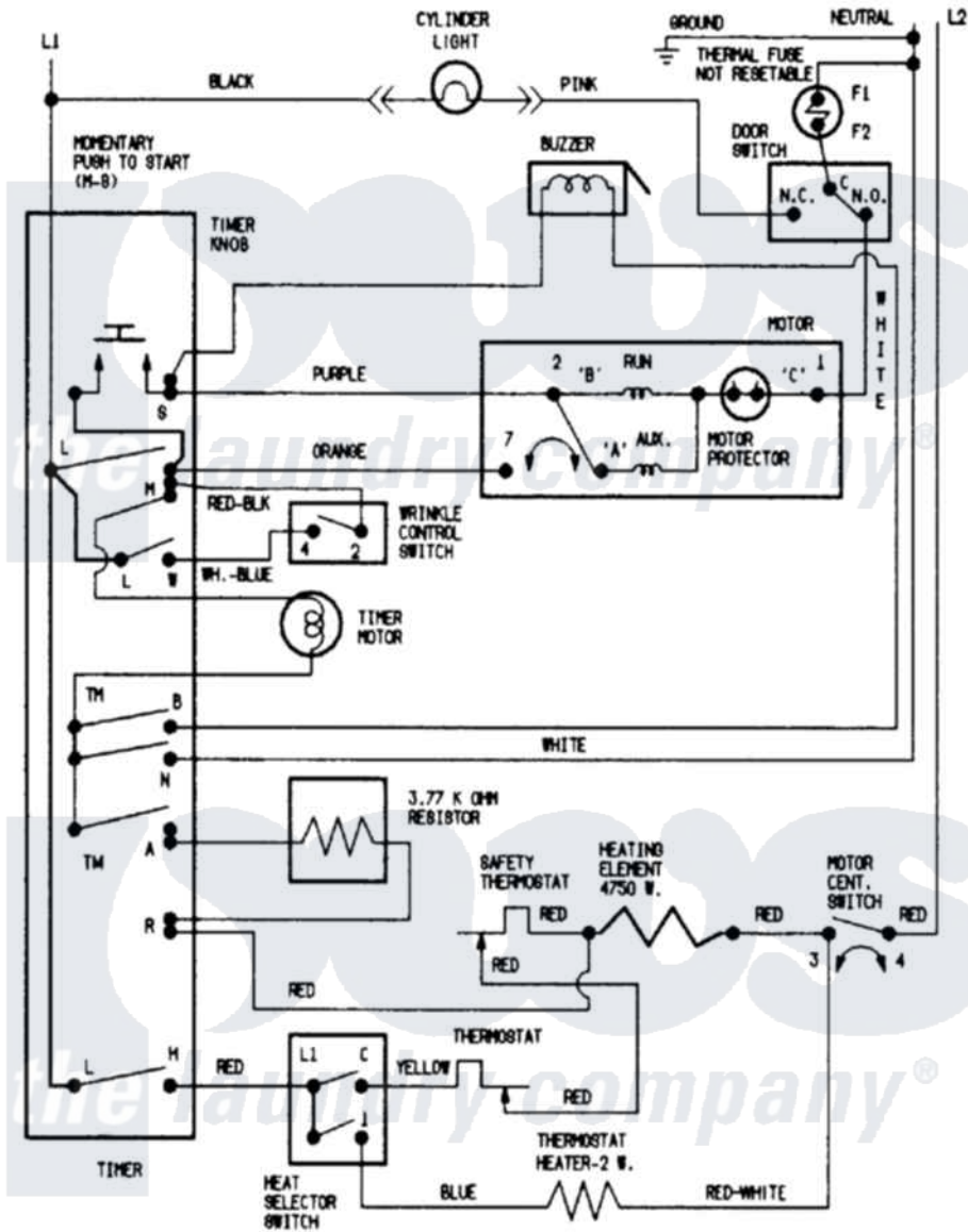
Maytag Residential Maytag PYE2000AYW Dryer Parts Parts Diagram 07 - WIRING INFORMATION Click on the part number to view part
