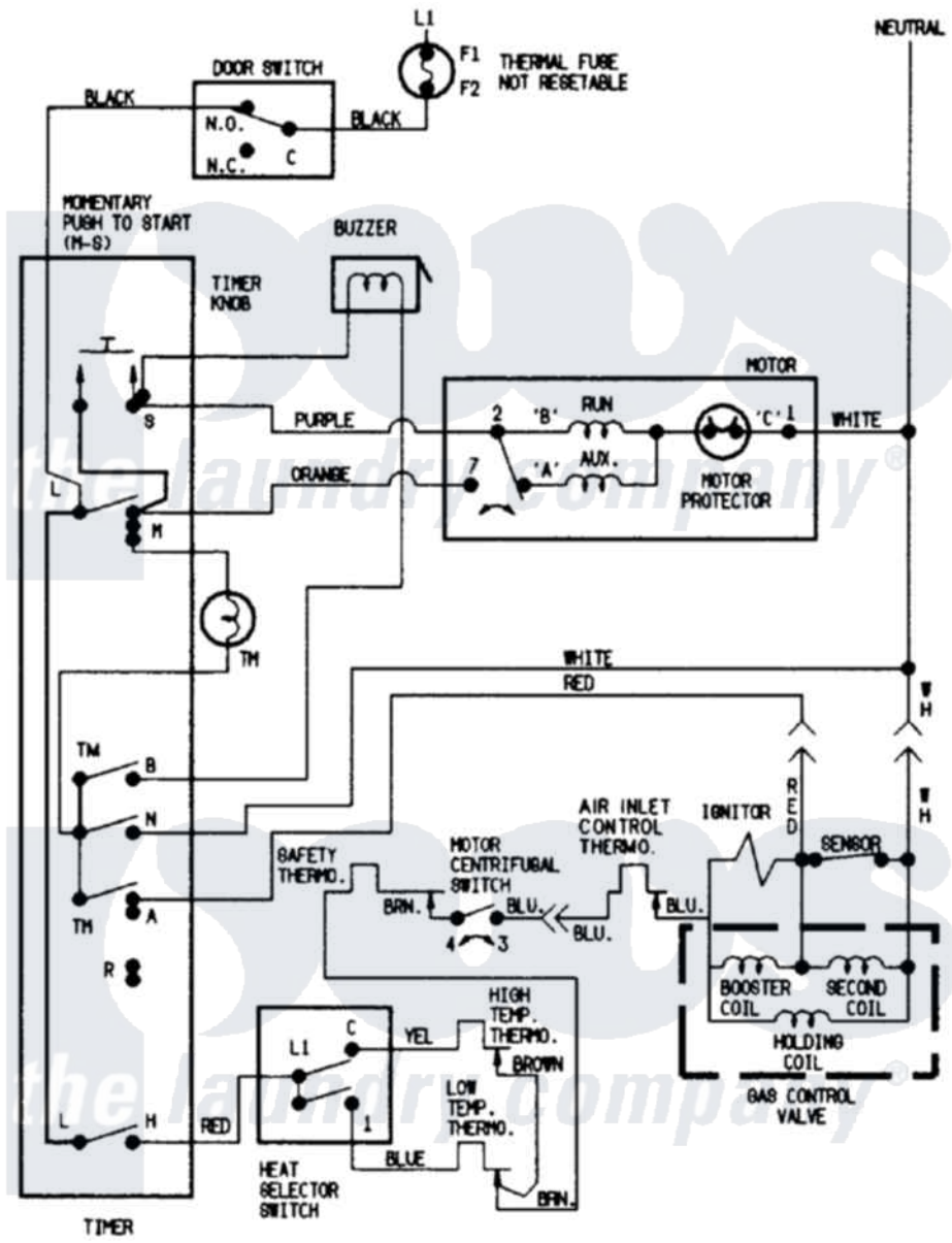
Norge Residential Norge DGN203A Dryer Parts Parts Diagram 05 - WIRING INFORMATION Click on the part number to view part
