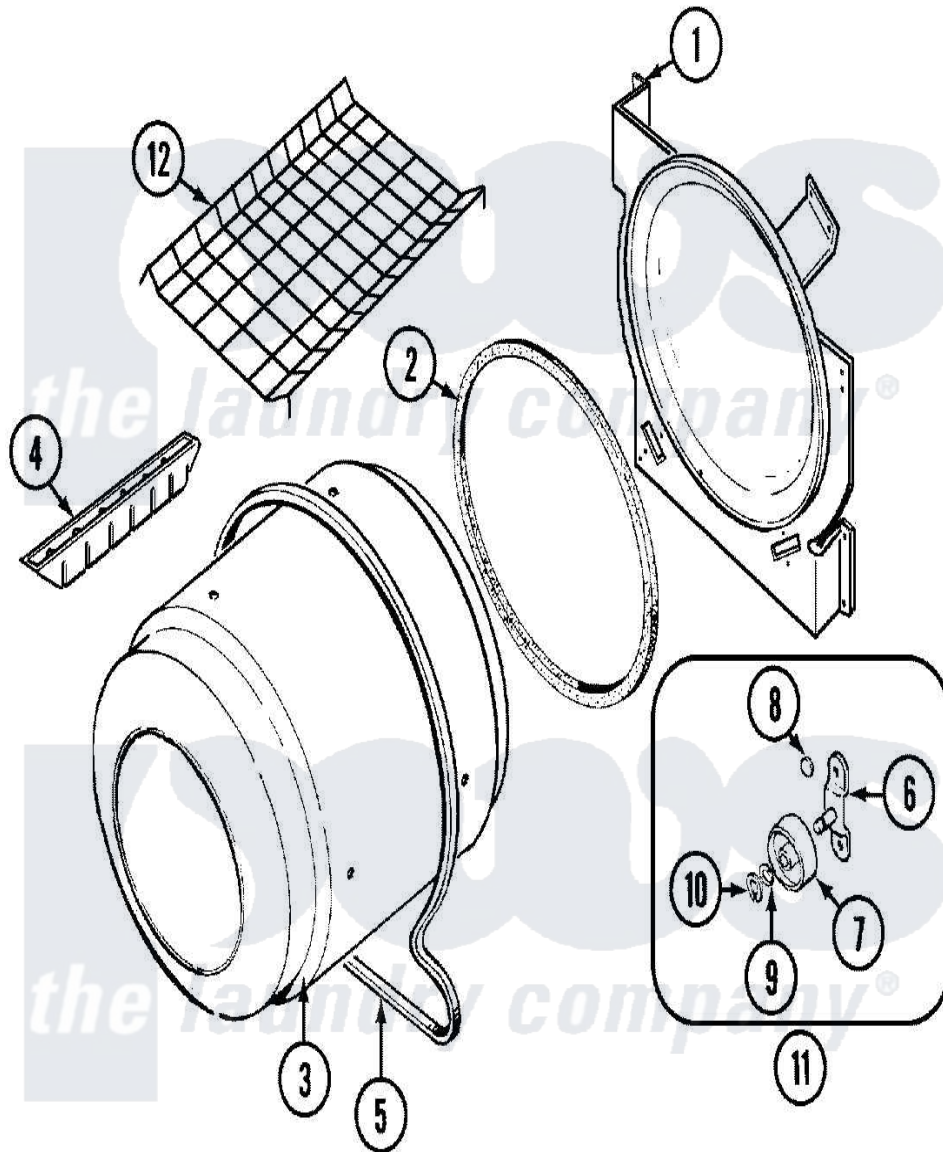
Norge Residential Norge DGN204A Dryer Parts Parts Diagram 06 - TUMBLER Click on the part number to view part
